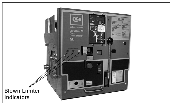
Figure 21.1 DSL-308
