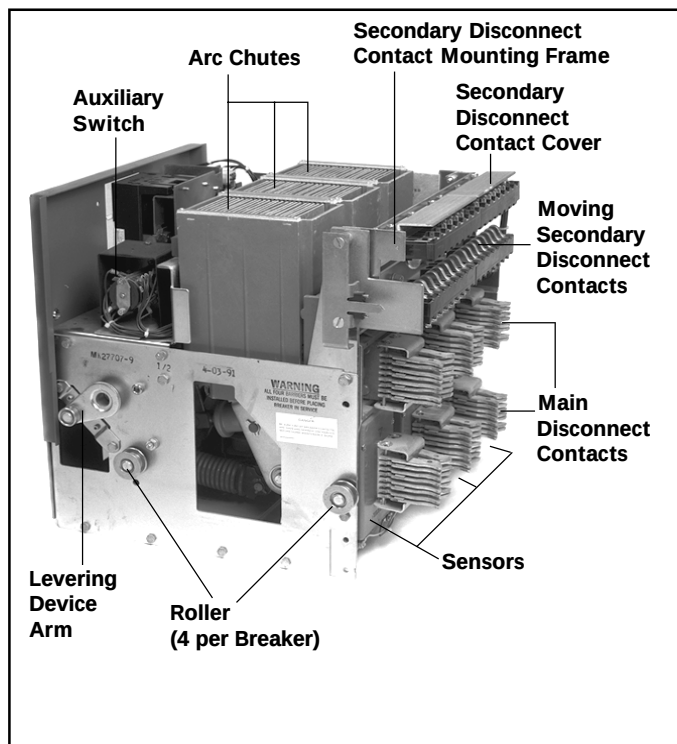
Figure 2.3 DS-416 Breaker Side View without Barriers
