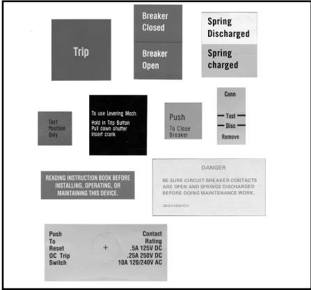
Figure 22.2 DS Breaker Label Kit Style Number 8187A84G01
