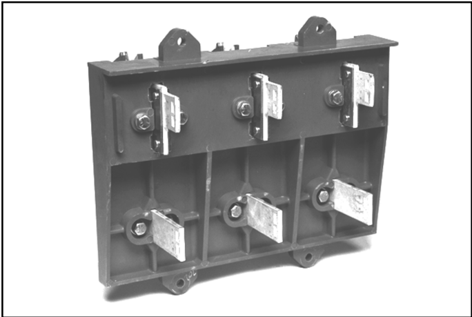
Figure 4.2 DS-206 Pole Unit Assembly
