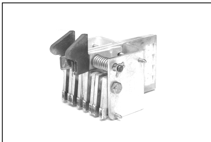
Figure 5.4 DS-416 Upper Stud Assembly
