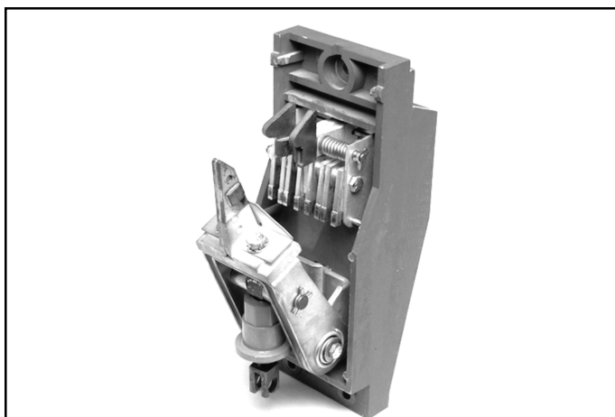
Figure 5.1 DS-840 Pole Unit Assembly
