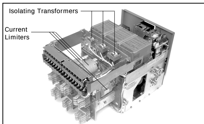
Figure 21.2 DSL-416 w/o barriers
