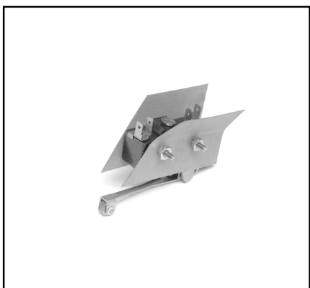
Figure 14.4 Latch Check Switch
