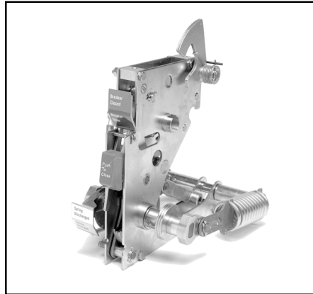
Figure 12.2 Manual Mechanism with Closing Spring
