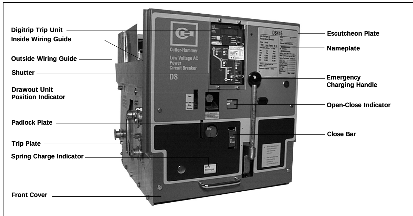
Figure 2.1 DS-416 Breaker Front View
